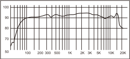
FREQ. RESPONSE (dB SPL, 1W, 1m)
